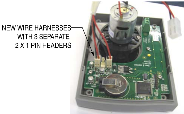
DR-2000 Main PCB.
